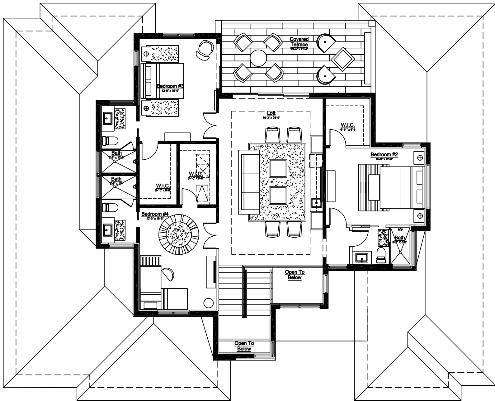
Second Floor Plan Scale \frac{1}{4}'' = 1'0''
